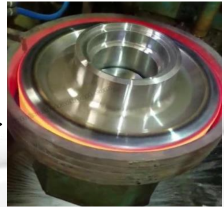
Surface Quenching >
